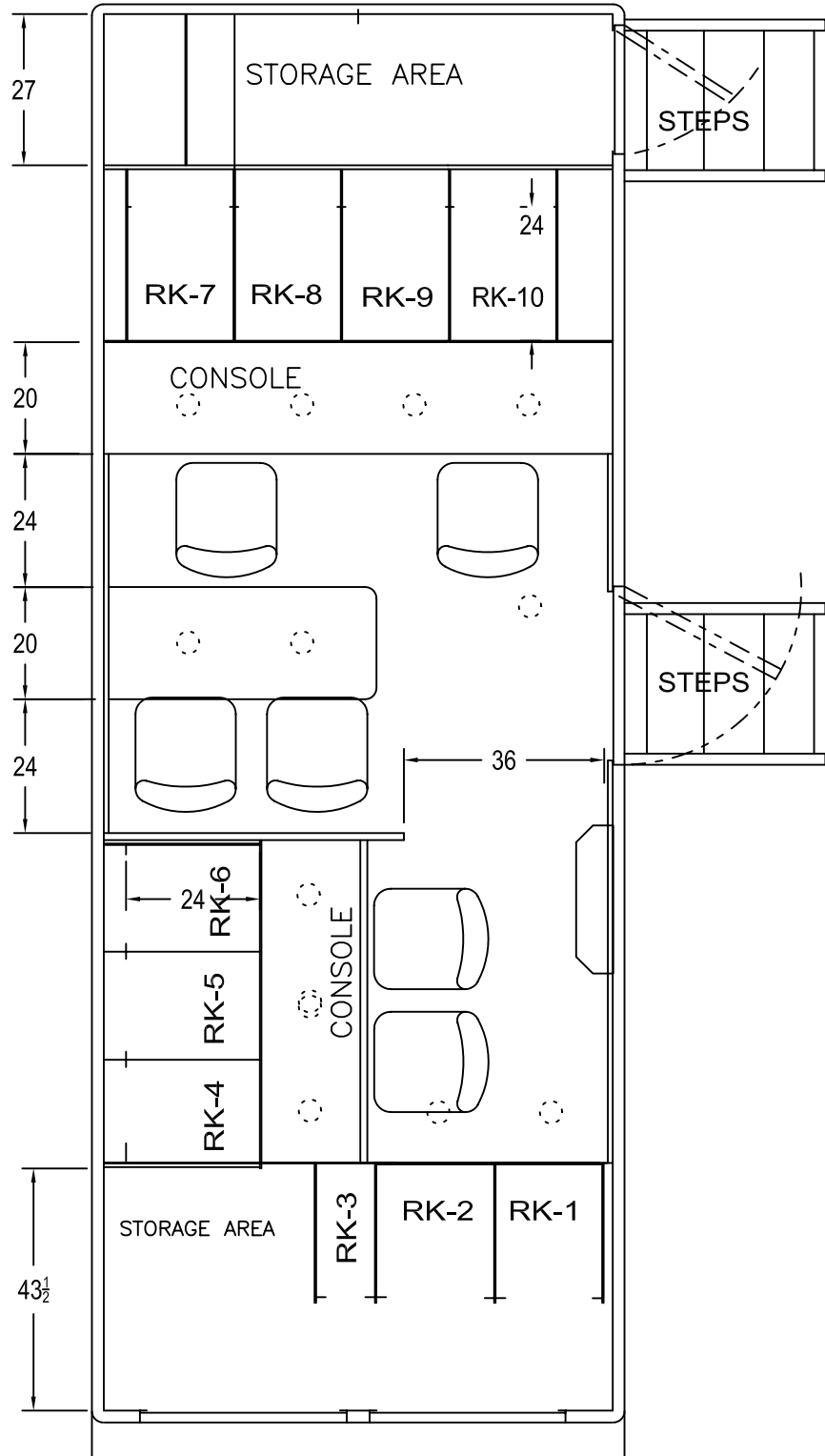
PLAN VIEW
